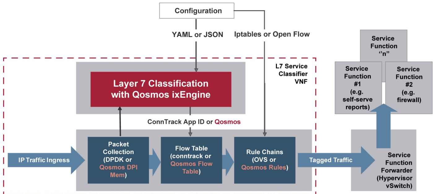
Reference architecture for L7-based Service Chaining built on Qosmos ixEngine
